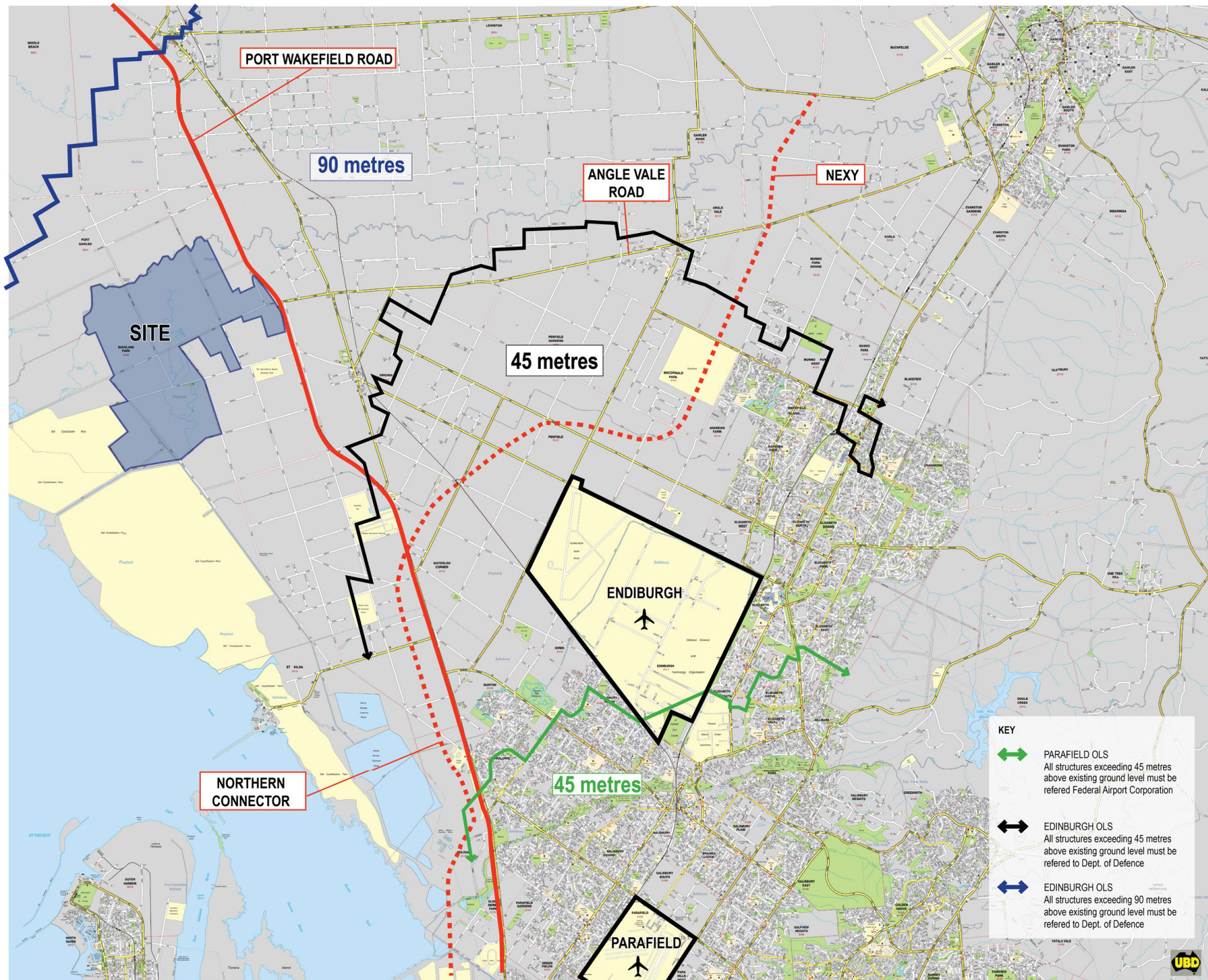
FIGURE 15.4 AIRPORTS - OBSTACLE LIMITATION SURFACES
